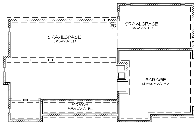
1 FOUNDATION PLAN A-3
